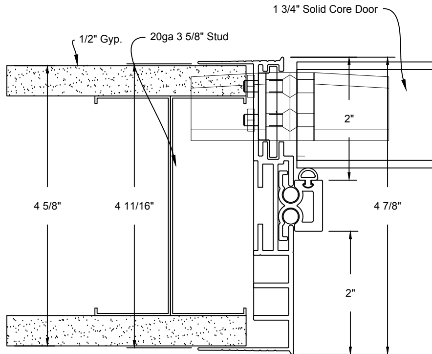
Minimalist Door Frame Concealed Hinge Detail
