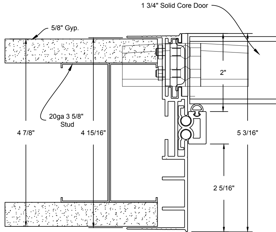
Minimalist Door Frame Concealed Hinge Detail
