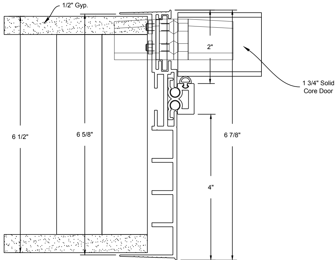
Minimalist Door Frame Concealed Hinge Detail
