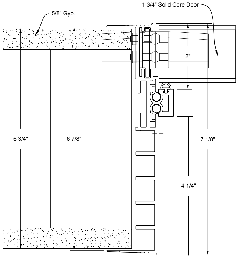
Minimalist Door Frame Concealed Hinge Detail
