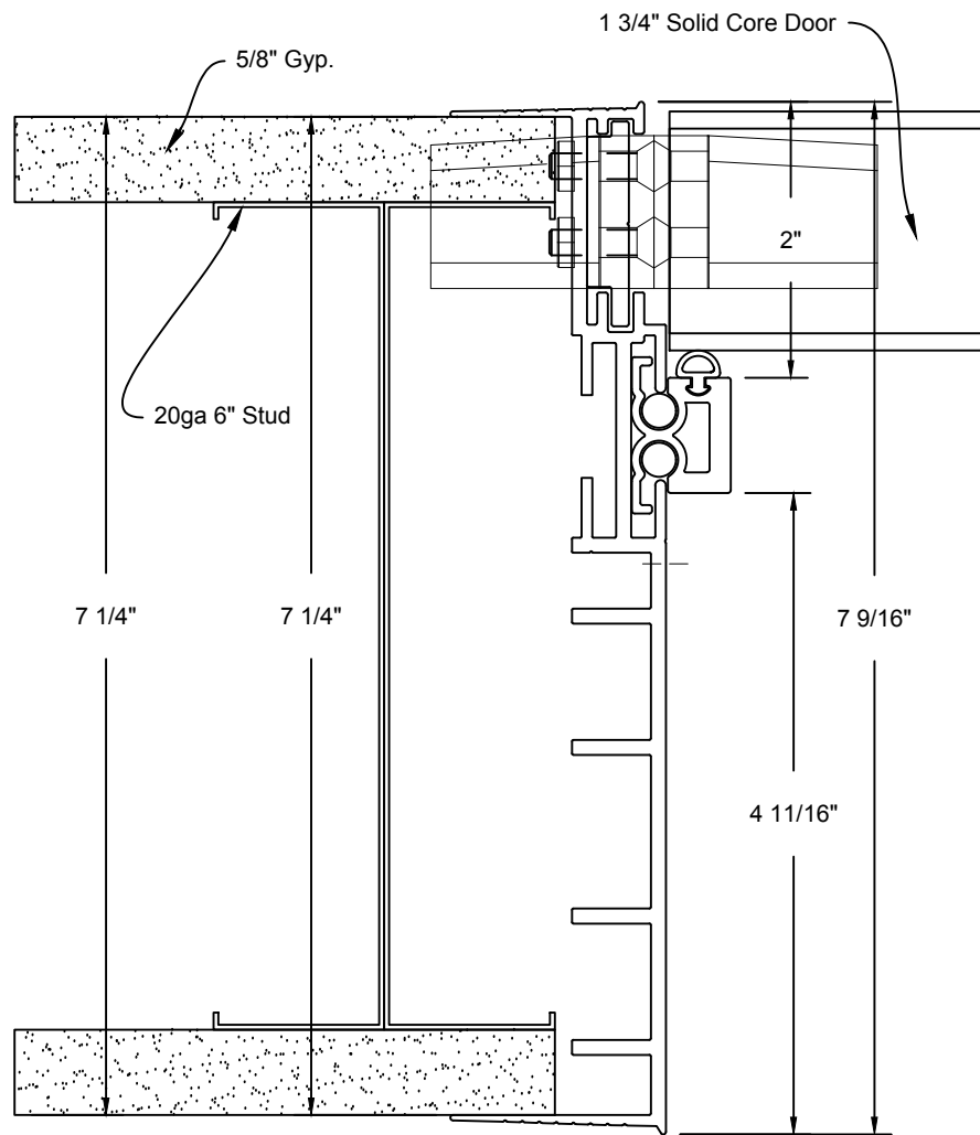
Minimalist Door Frame Concealed Hinge Detail
