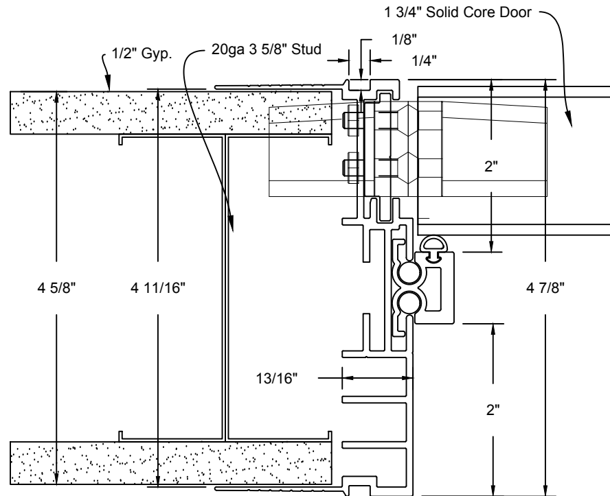
Minimalist Door Frame w/ Reveal Concealed Hinge Detail
