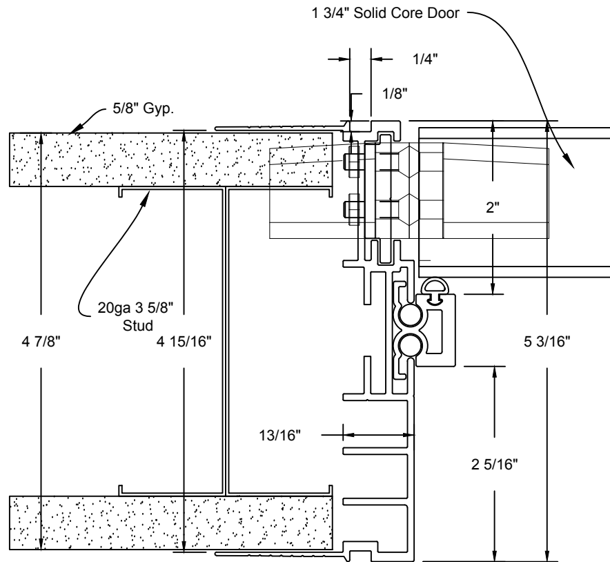
Minimalist Door Frame w/ Reveal Concealed Hinge Detail
