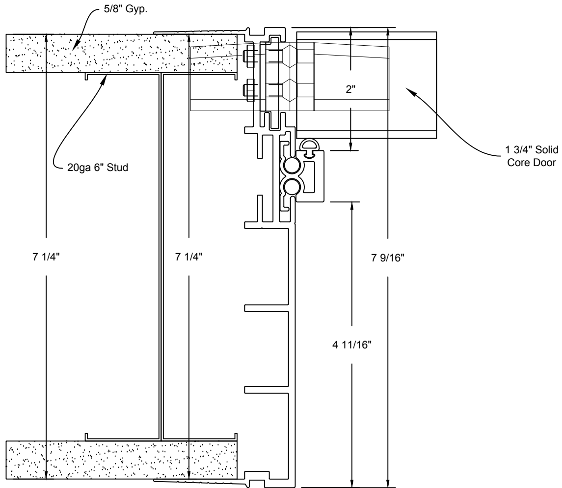
Minimalist Door Frame Concealed Hinge Detail
