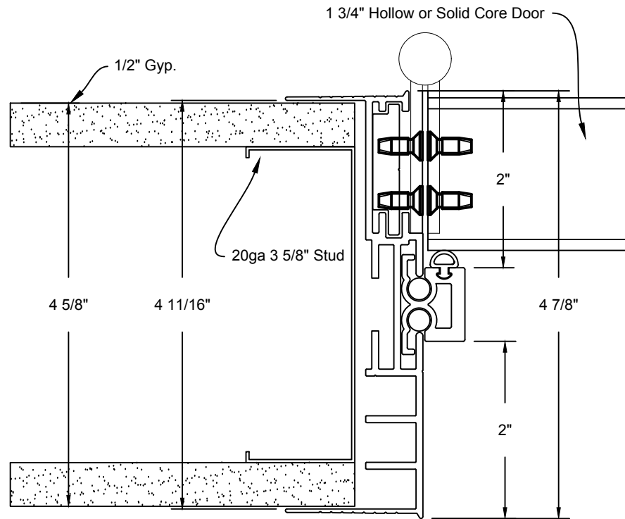
Minimalist Door Frame Hinge Detail
