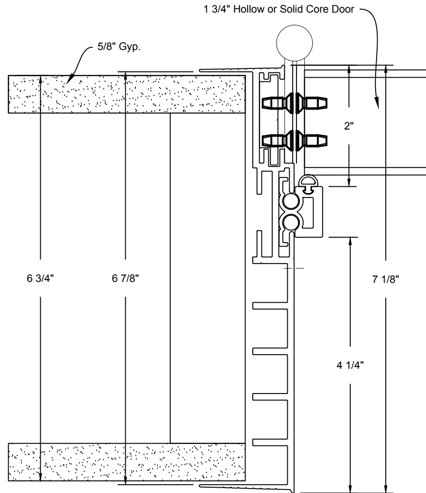
Minimalist Door Frame Hinge Detail
