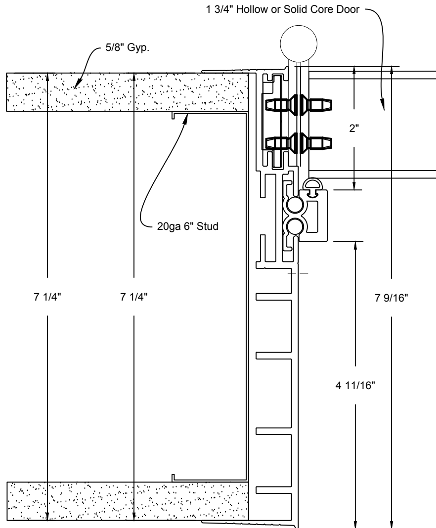
Minimalist Door Frame Hinge Detail
