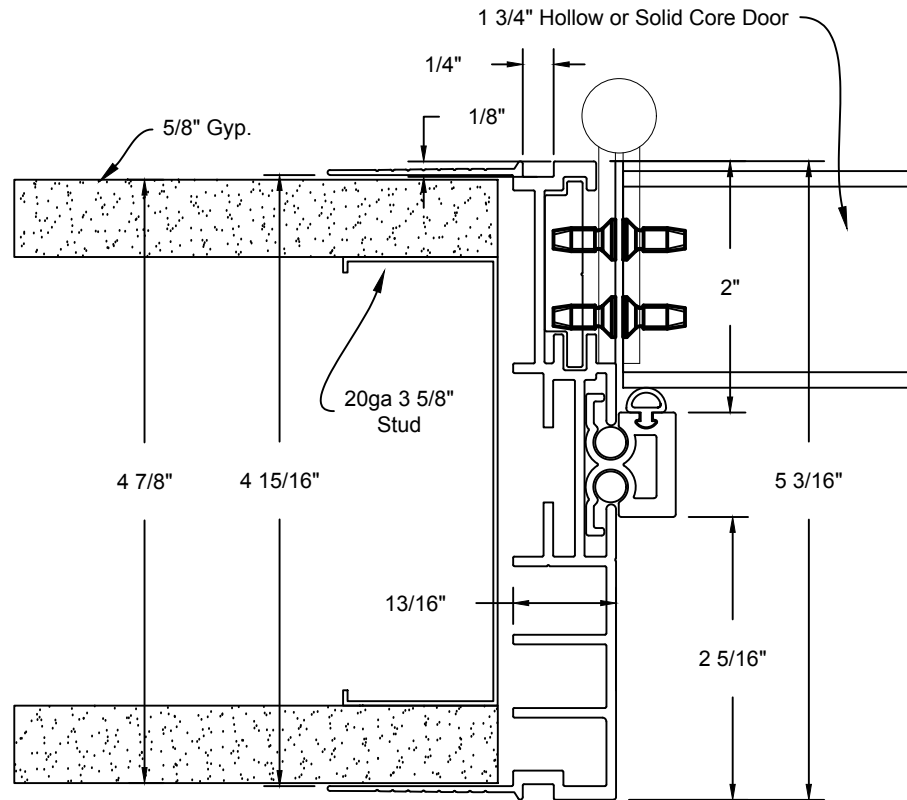
Minimalist Door Frame w/ Reveal Hinge Detail
