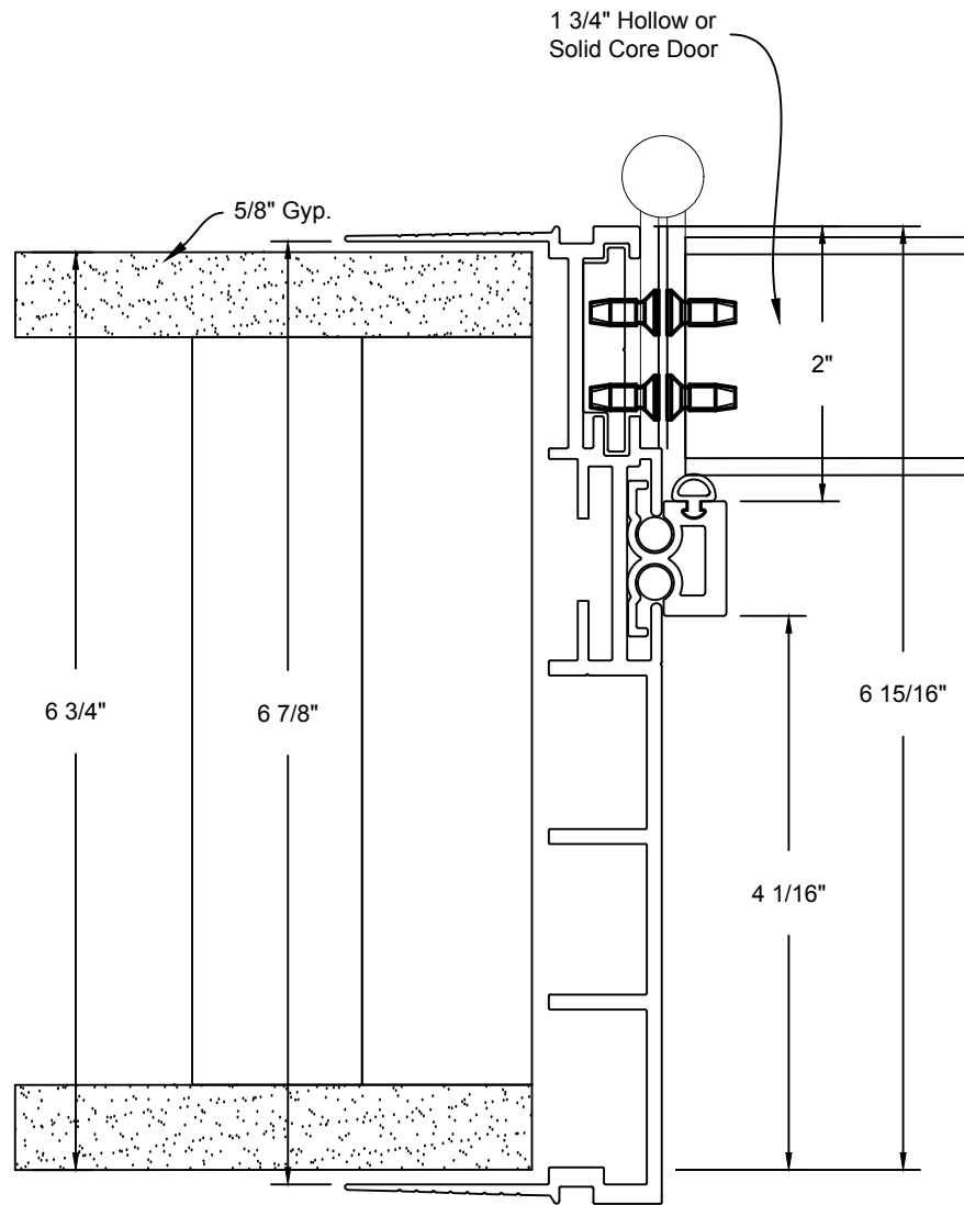
Minimalist Door Frame Hinge Detail
