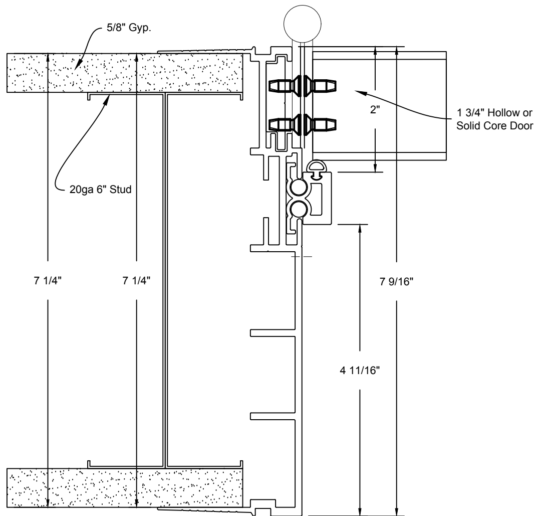
Minimalist Door Frame Hinge Detail
