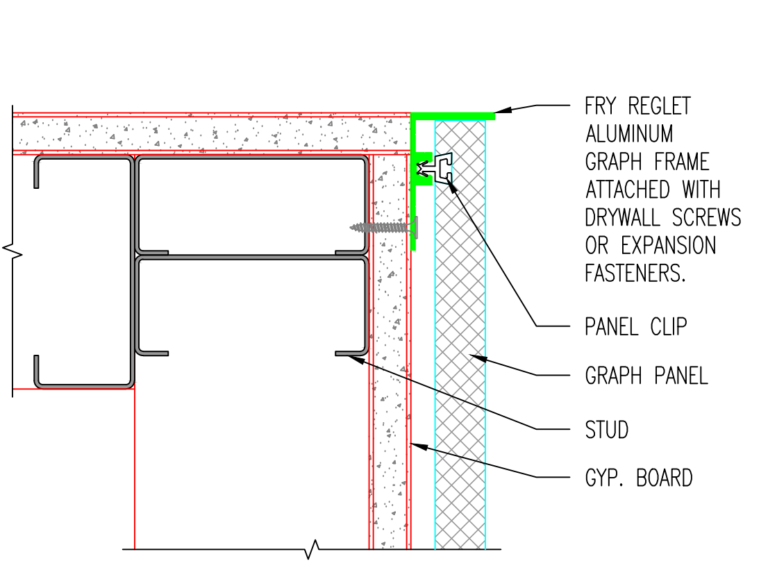
K CORNER TERMINATION DETAIL-3/4" PANEL SCALE: NTS
