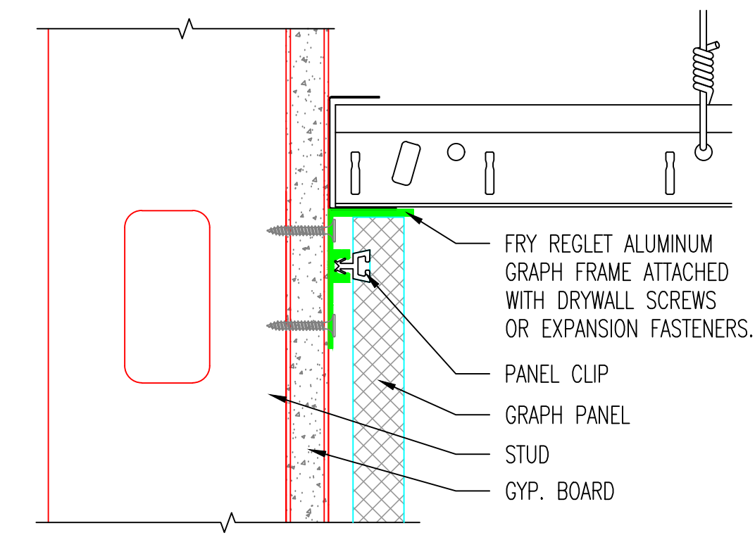
C CEILING TERMINATION DETAIL-3/4" PANEL SCALE: NTS
