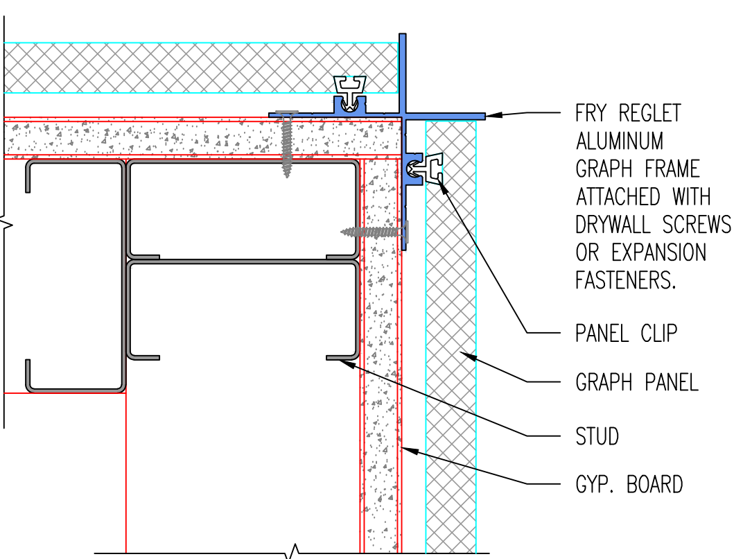
O X CORNER DETAIL-3/4" PANEL SCALE: NTS
