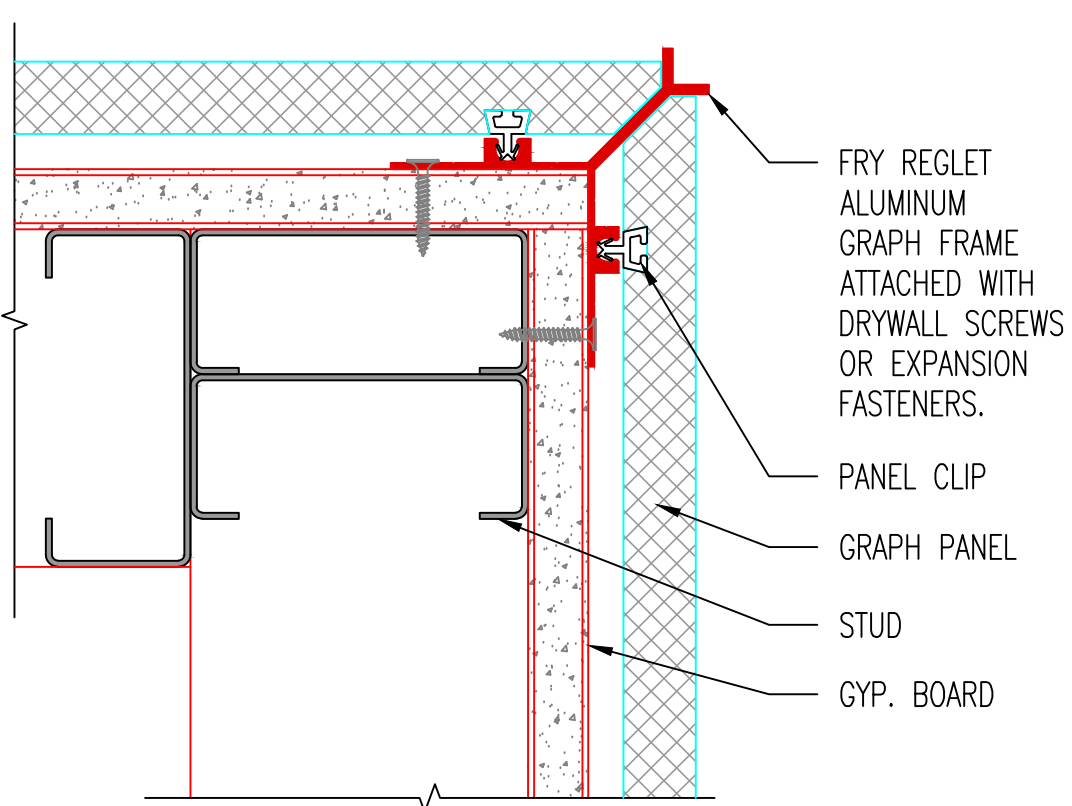
M OPEN CORNER DETAIL-3/4" PANEL SCALE: NTS
