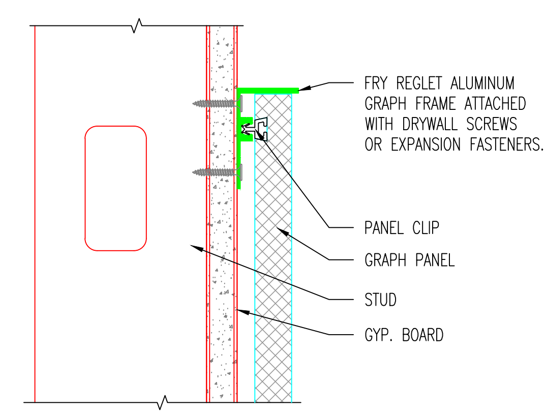
H TERMINATION DETAIL-3/4" PANEL SCALE: NTS
