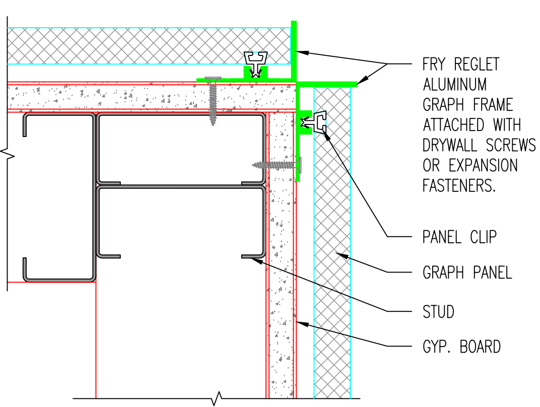
G OUTSIDE CORNER DETAIL-3/4" PANEL SCALE: NTS
