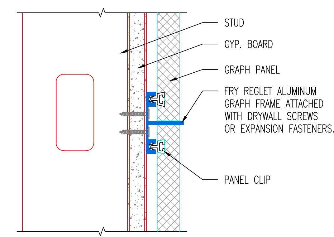
B PANEL RETAINER DETAIL-3/4" PANEL SCALE: NTS
