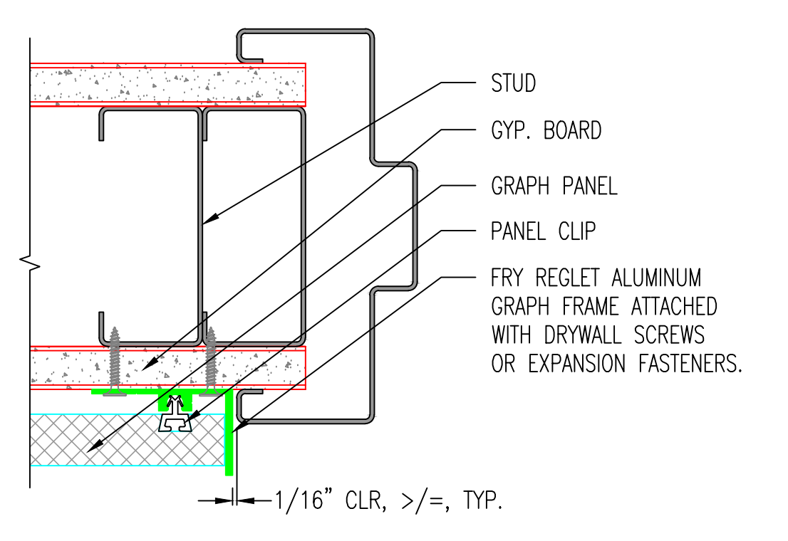
E JAMB DETAIL-3/4" PANEL SCALE: NTS
