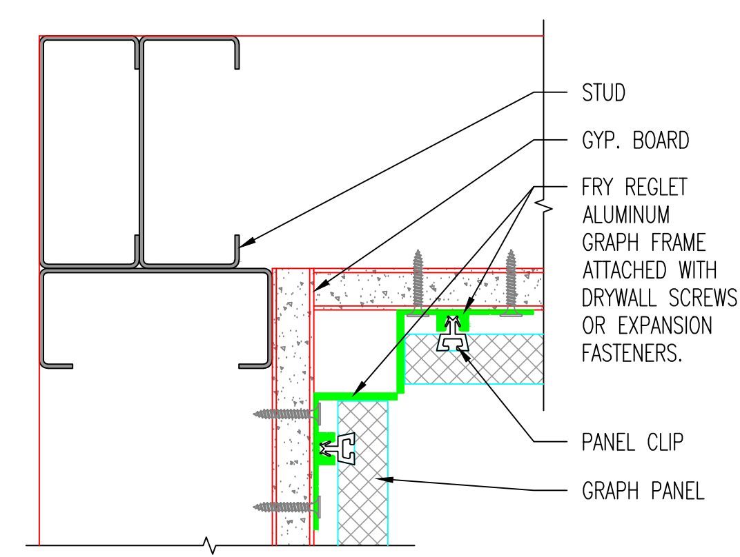
F INSIDE CORNER DETAIL-3/4" PANEL SCALE: NTS
