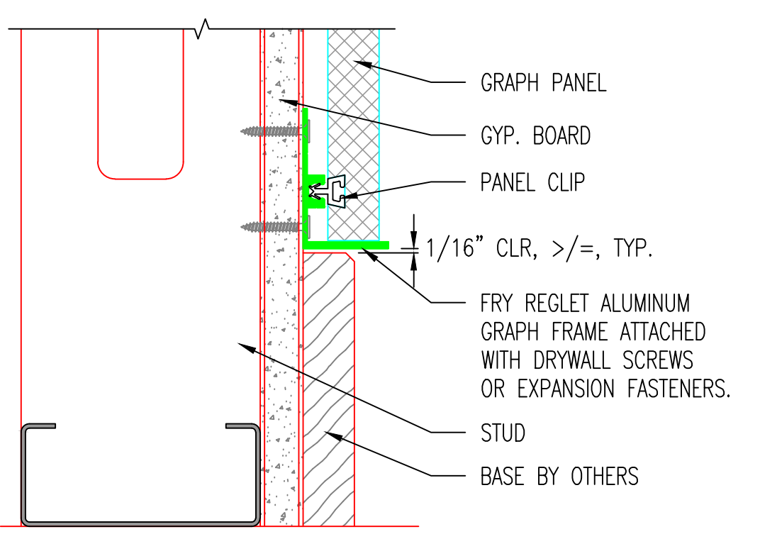
D TERMINATION AT BASE DETAIL-3/4" PANEL SCALE: NTS
