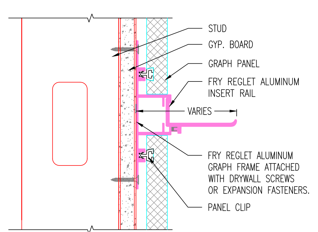
P INTEGRATED FUNCTIONAL REVEAL (IFR) DETAIL SCALE: NTS
