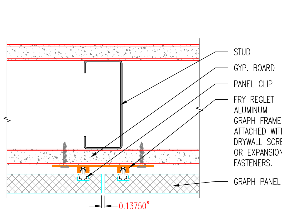
L BUTT REVEAL DETAIL-3/4" PANEL SCALE: NTS
