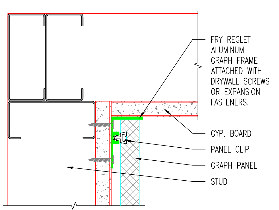
J INSIDE CORNER TERMINATION DETAIL-3/4" PANEL SCALE: NTS
