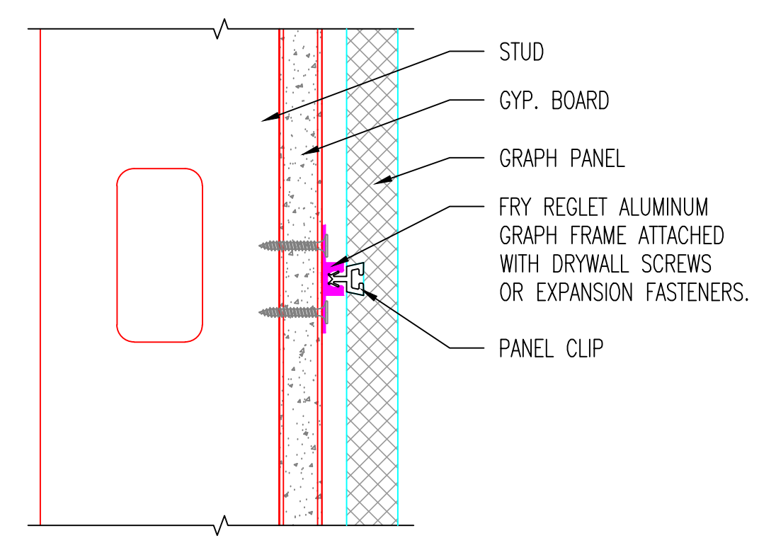
A INTERMEDIATE RETAINER DETAIL-3/4" PANEL SCALE: NTS
