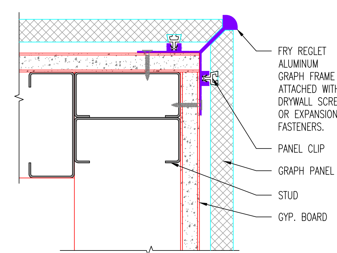
N BULLNOSE CORNER DETAIL-3/4" PANEL SCALE: NTS
