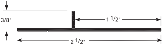
SPECIAL REVEAL MOLDING / PART NO. "T" PIECE
