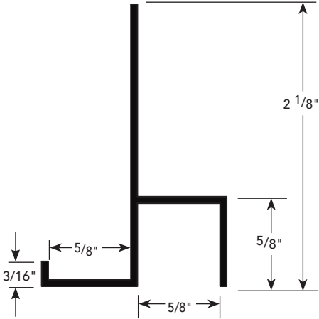
SPECIAL REVEAL MOLDING / PART NO. "T" PIECE
